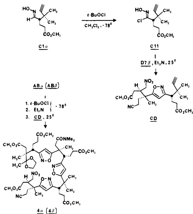
Scheme XIV
