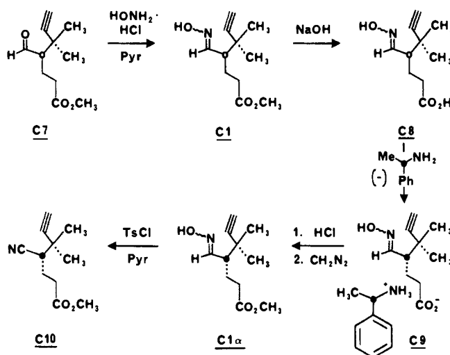
Scheme XII
