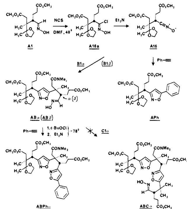
Scheme XIII
