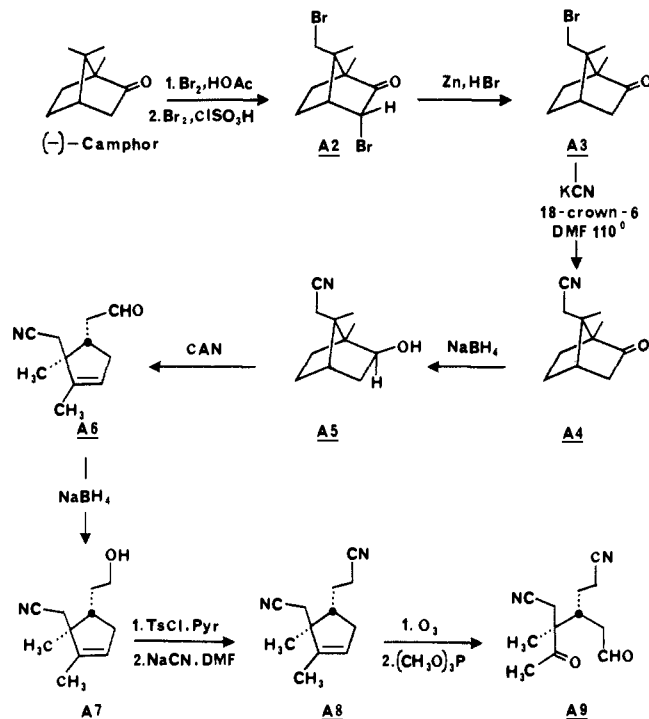
Scheme IV
